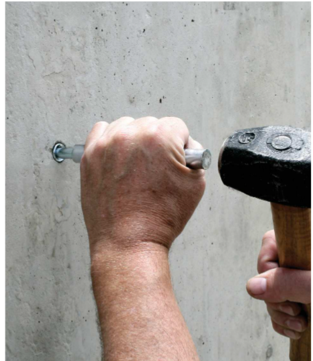
Anchor being set with hand setting tool.
