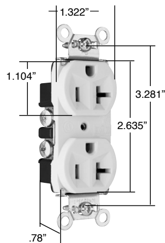
Dimensions for 15 & 20 Amp
