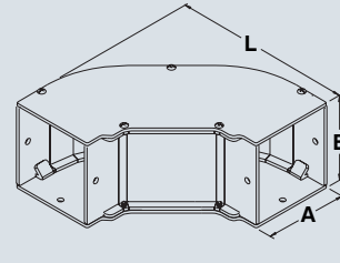
Elbow sweep 90 degrees
