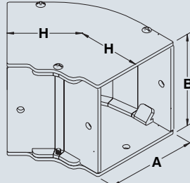
Elbow 45 degrees
