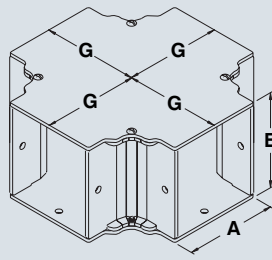
Cross fitting
