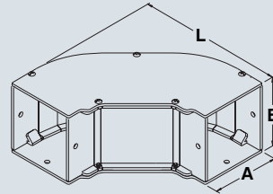
Elbow sweep 90 degrees
