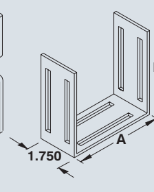
Joiner plate
