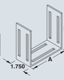
Joiner plate
