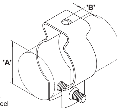
FIGURE 7310 - Rigid/EMT Clamp
