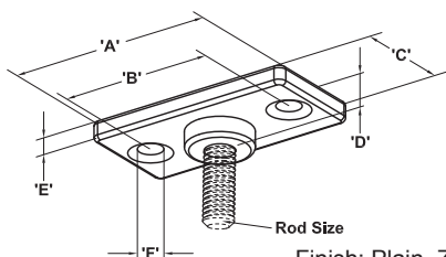
FIGURE 7502 - Beam Ceiling Flange
