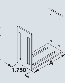
Joiner plate
