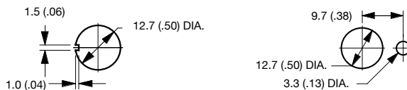
Mounting Hole With Keyway
