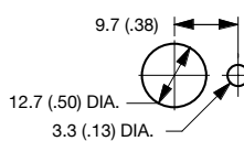
Mounting Hole With Locking Ring
