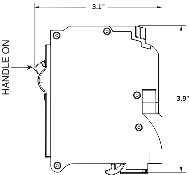
Single Pole
