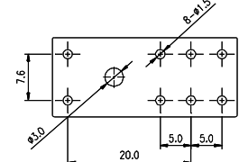
SQ2V-63 PCB pin layout
