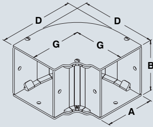
Elbow 90 degrees
