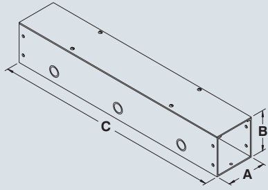
Straight section
