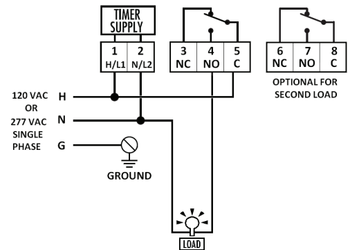
TYPICAL SPST WIRING - LOAD SAME VOLTAGE AS TIMER SUPPLY
