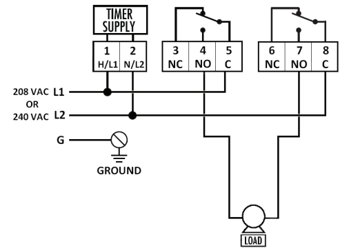
TYPICAL DPST WIRING - LOAD SAME VOLTAGE AS TIMER SUPPLY
