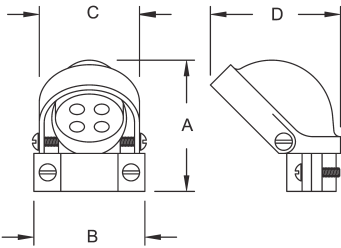
A = Height B = Width of clamp C = Width of head D = Depth of head
