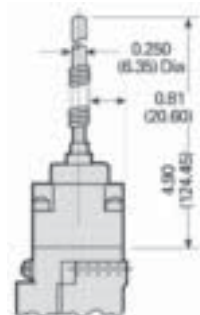
Wobble head with nylon head 3SE03-DW1 3SX03-KW2
