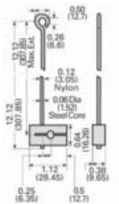
Nylon Covered Wire Actuator 3SX03-KL533
